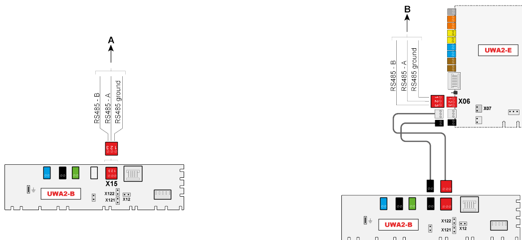
Modbus connecting (A) with a standard Brink HRA with only fitted the PCB UWA2-B
